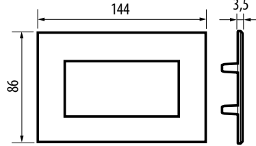
HW4804...
